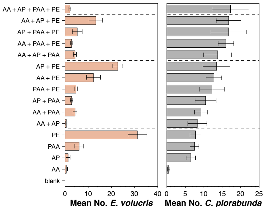
Comparison of trap capture of the syrphid fly, Eupeodes volucris and the lacewing, Chrysoperla plorabunda in the large factorial experiment evaluating all possible combinations of AA, AP, PAA, and PE. Dotted lines within a graph separate one, two, three and four component blends.
